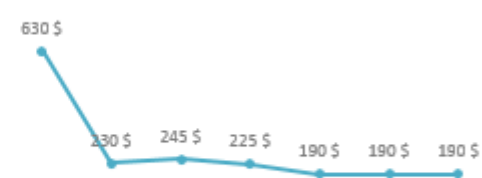
Indium
