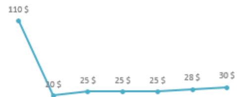
Tellure
