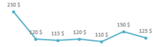
Gallium
